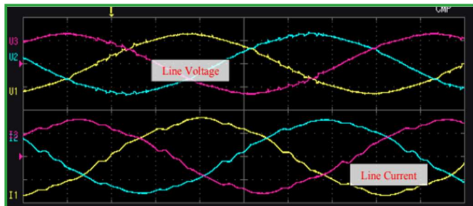
Figure 3: Conventional VFD with filters: Input voltage and current waveforms
