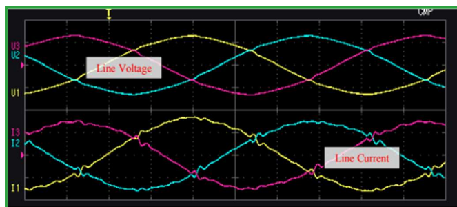
Figure 1: Clean Power VFD Input current and voltage
