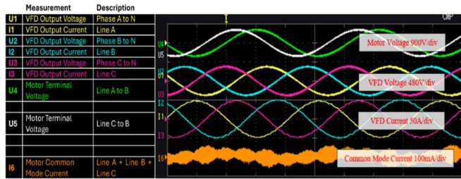
Figure 1: Clean Power VFD output signals
