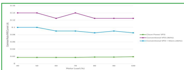
Figure 3: Common mode current (RMS) comparison
