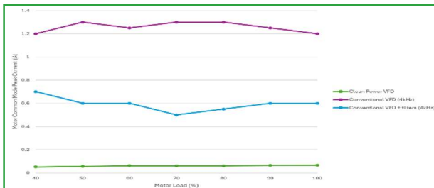
Figure 2: Common mode peak current comparison
