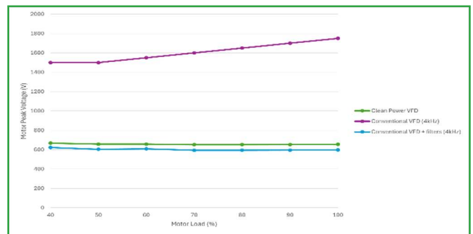
Figure 4: Motor peak voltage (V)
